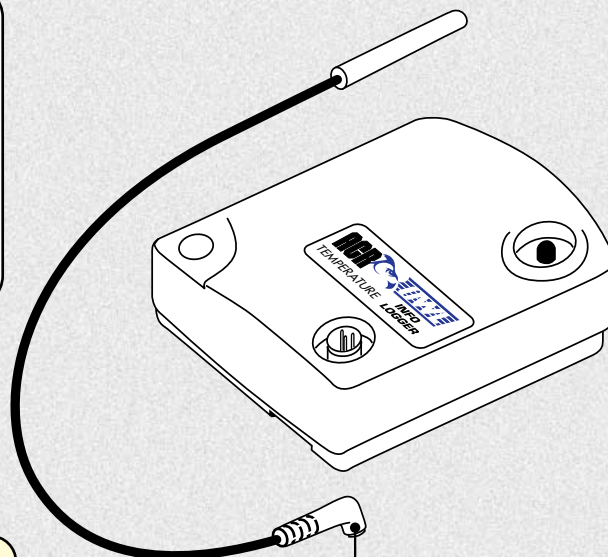
OWL ET series temperature probe. (Order separately).
